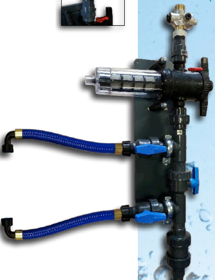
With optional pressure gauge
